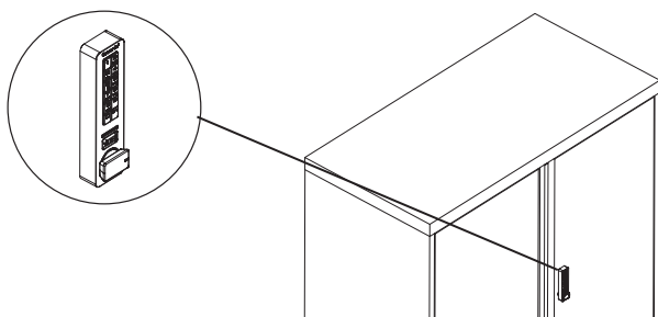
Vertical installation
